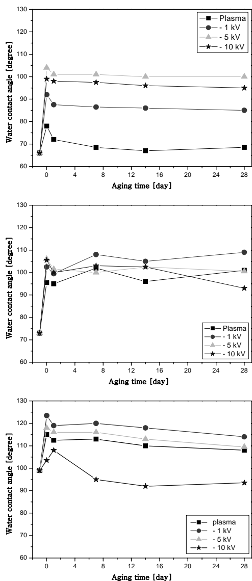
Fig. 1 Water contact angle of CF 4 PSII treated (a) EVOH (b) LLDPE and (c) PET film with varying ion energy as a function of aging time. Treatment condition of plasma is: 0 kV, 1 mTorr, and 200 W.
