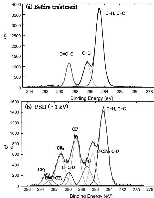
Fig. 2 XPS spectrum of PET films (a) untreated and (b) treated by PSII
